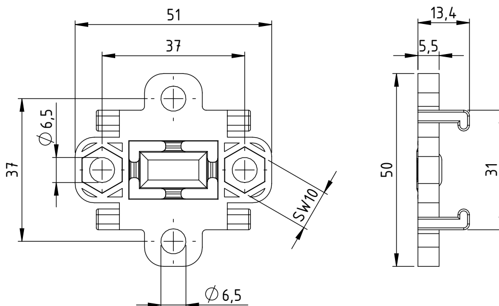
Fig. 10: Support standard
